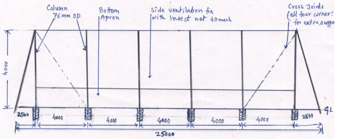
SIDE VIEW
